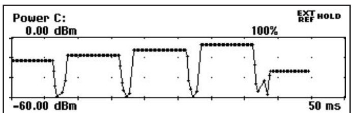
Figure 7: Power step (close up)
